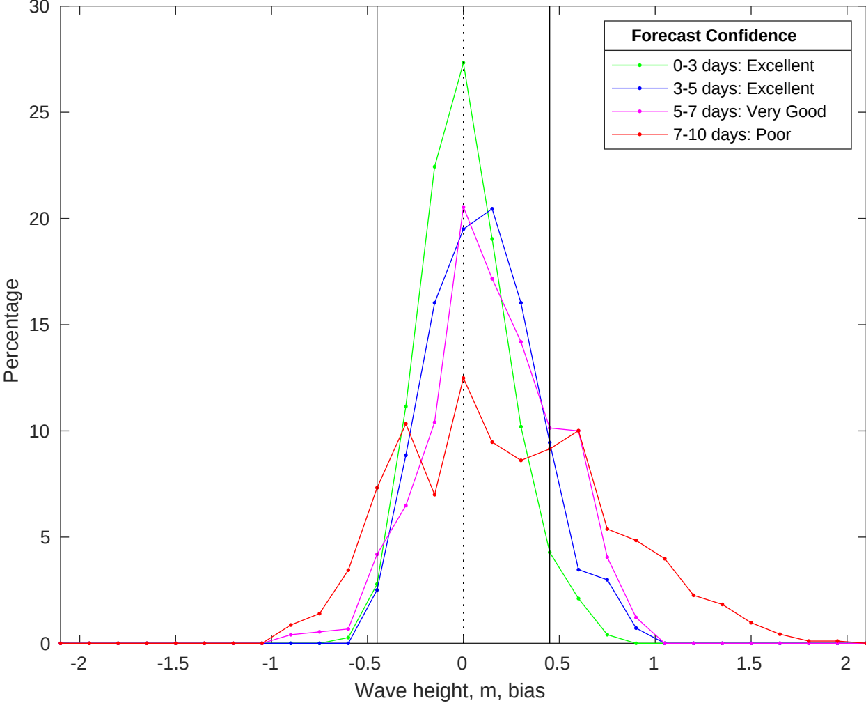
NDBC 46069 vs CMEMS Waves Bias Histogram: 24-Jun-2025
