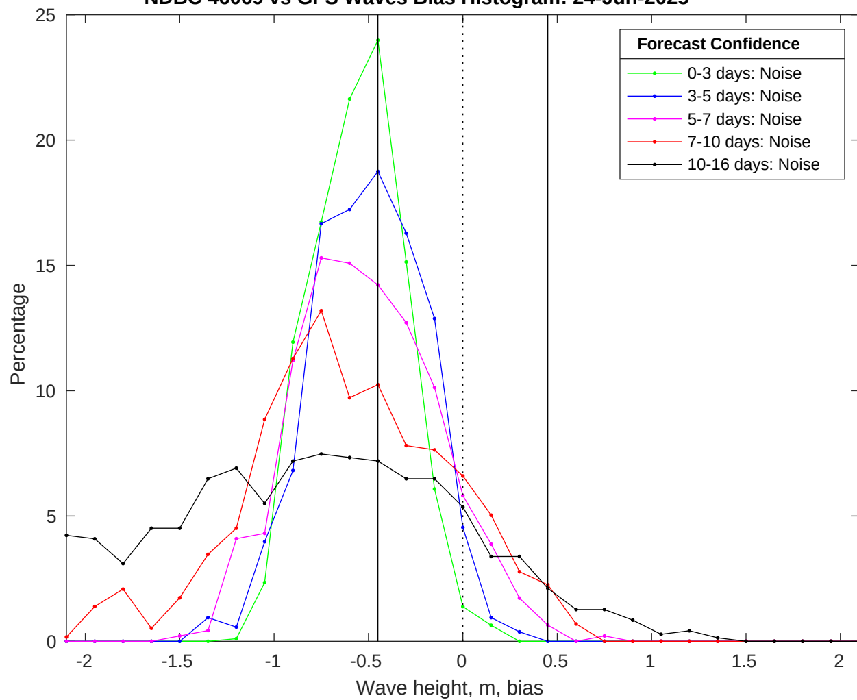
NDBC 46069 vs GFS Waves Bias Histogram: 24-Jun-2025
