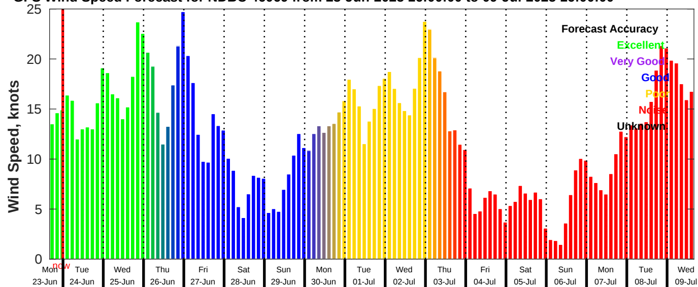
GFS Wind Speed Forecast for NDBC 46069 from 23-Jun-2025 16:00:00 to 09-Jul-2025 16:00:00
