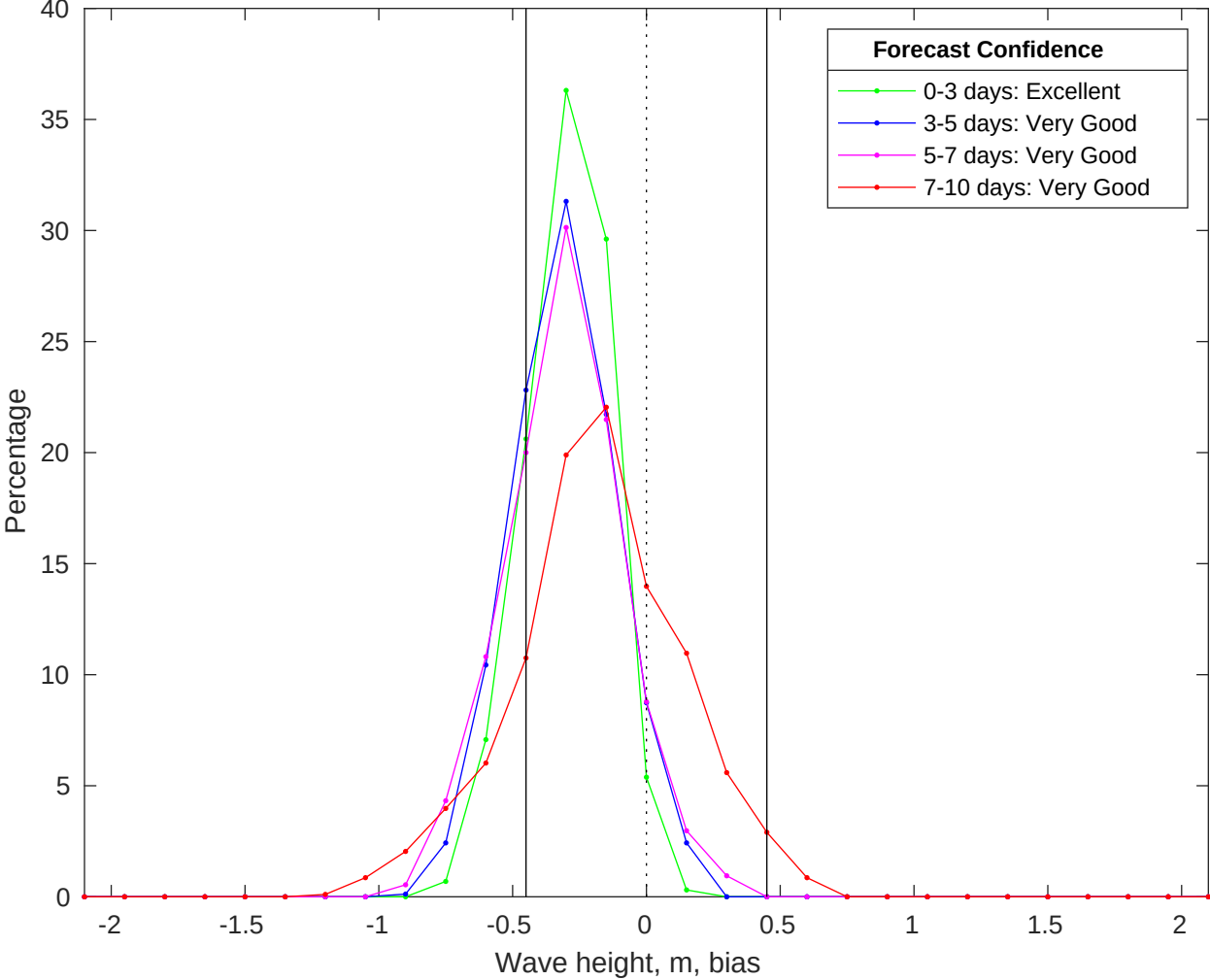
NDBC 51209 vs CMEMS Waves Bias Histogram: 24-Jun-2025
