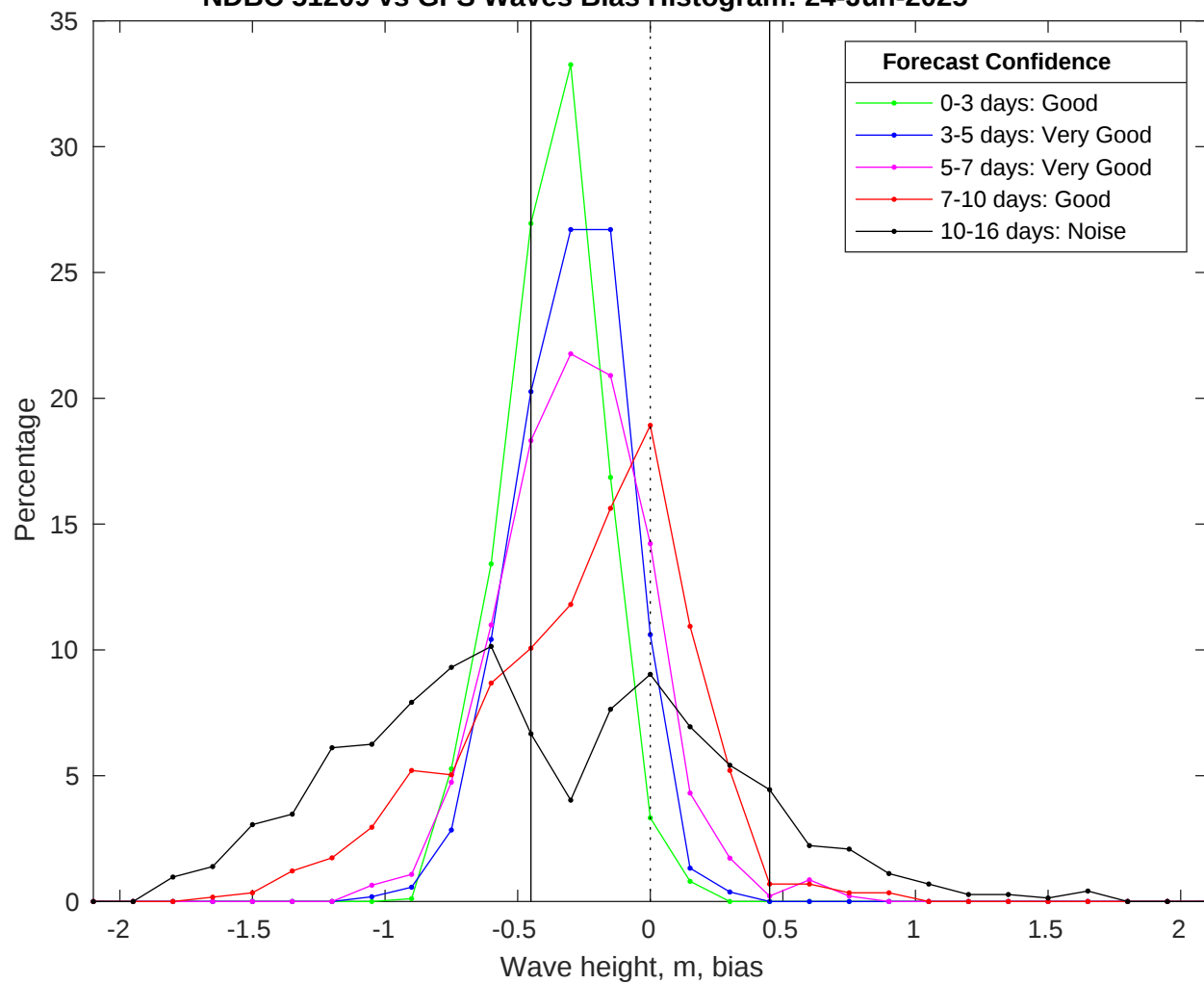
NDBC 51209 vs GFS Waves Bias Histogram: 24-Jun-2025
