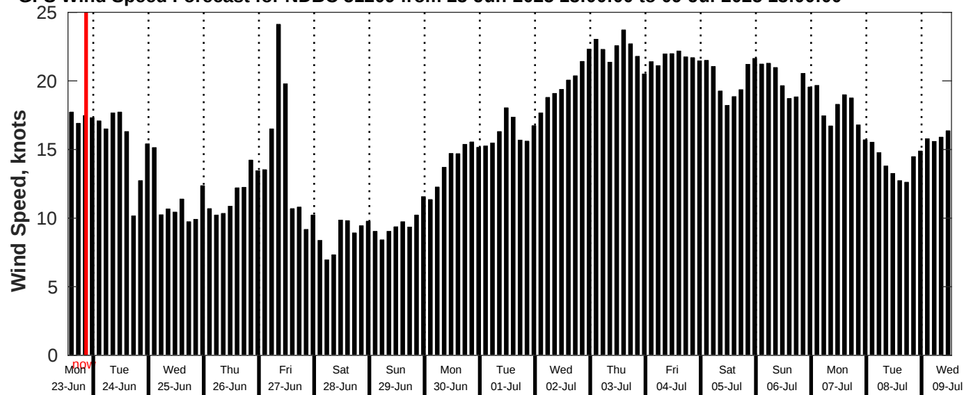
GFS Wind Speed Forecast for NDBC 51209 from 23-Jun-2025 13:00:00 to 09-Jul-2025 13:00:00
