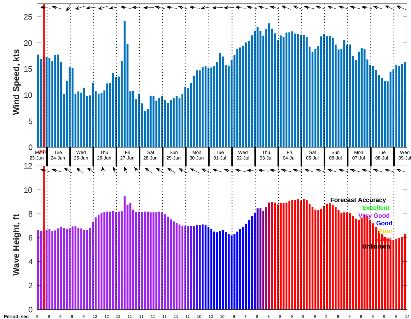
Wind & Wave Forecast for NDBC 51209 from 23-Jun-2025 13:00:00 to 09-Jul-2025 13:00:00
