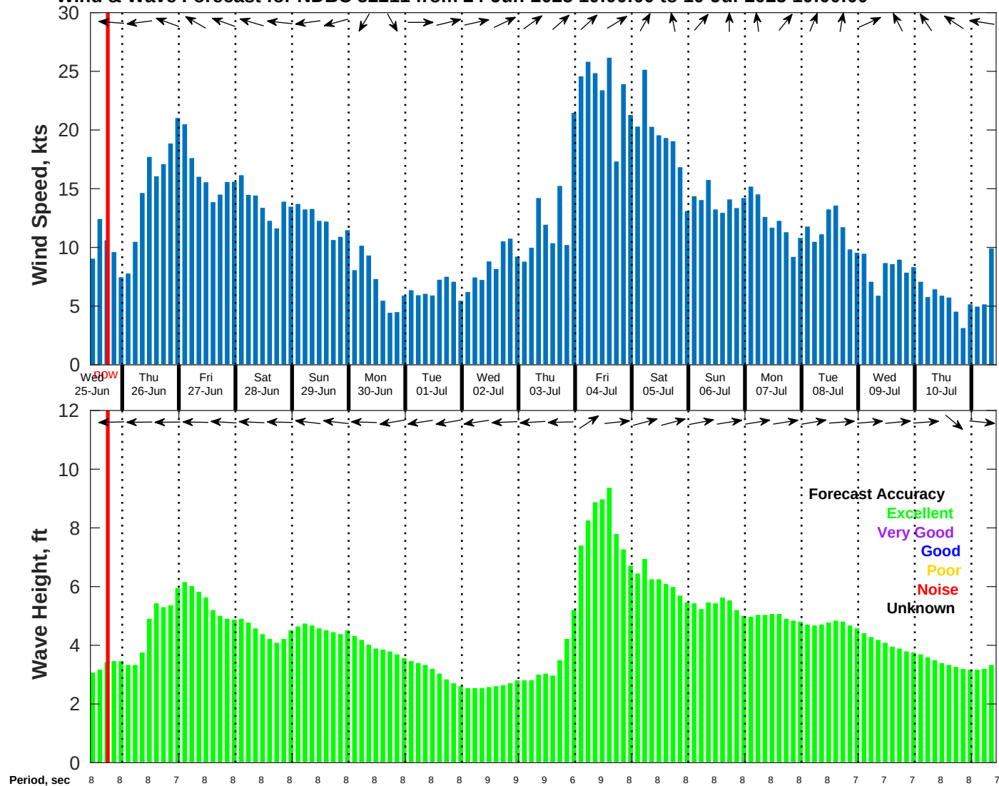
Wind & Wave Forecast for NDBC 52211 from 24-Jun-2025 10:00:00 to 10-Jul-2025 10:00:00
