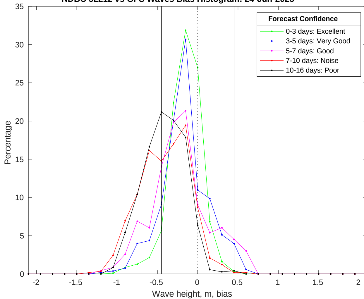
NDBC 52212 vs GFS Waves Bias Histogram: 24-Jun-2025
