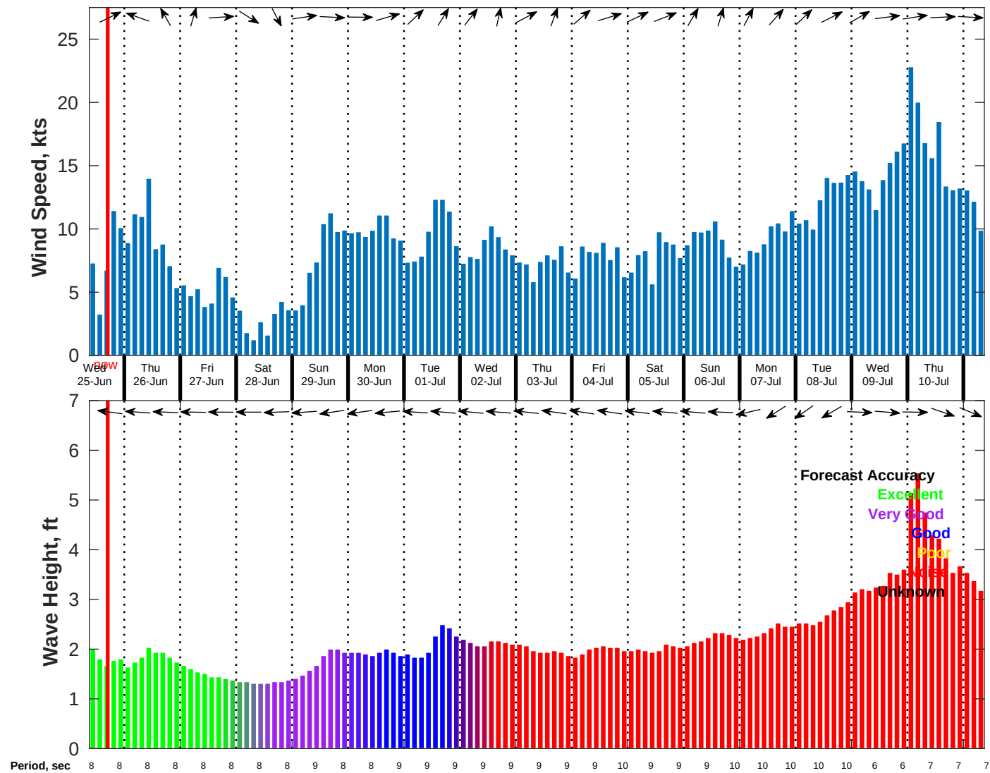
Wind & Wave Forecast for NDBC 52212 from 24-Jun-2025 09:00:00 to 10-Jul-2025 09:00:00
