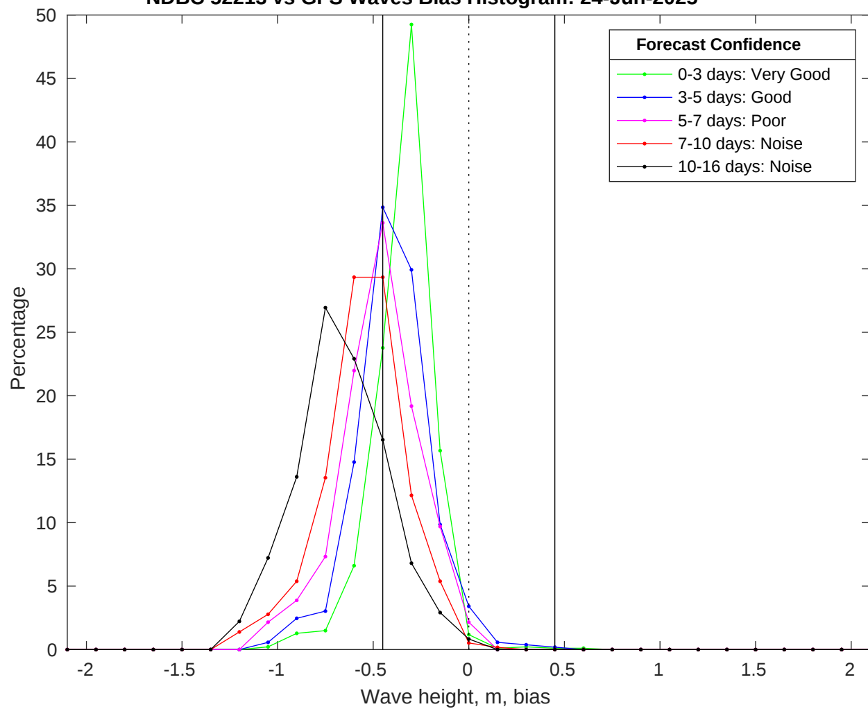
NDBC 52213 vs GFS Waves Bias Histogram: 24-Jun-2025
