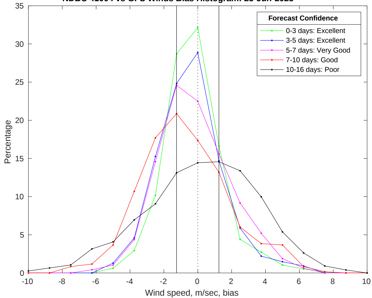
NDBC 41004 vs GFS Winds Bias Histogram: 25-Jun-2025
