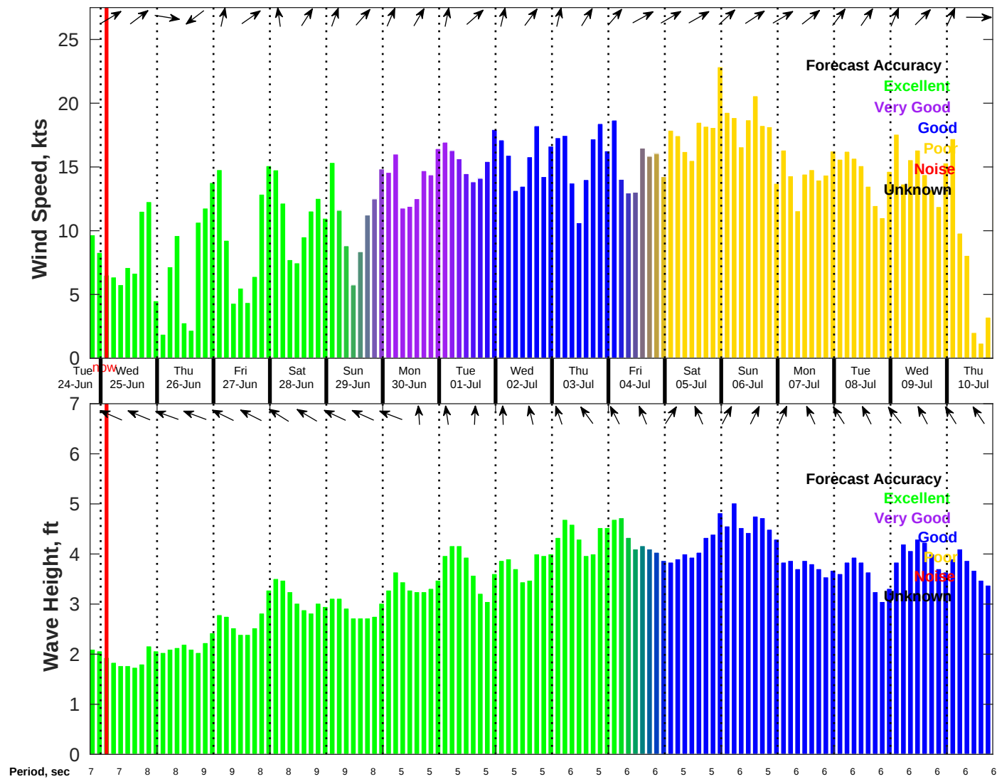
Wind & Wave Forecast for NDBC 41004 from 24-Jun-2025 19:00:00 to 10-Jul-2025 19:00:00
