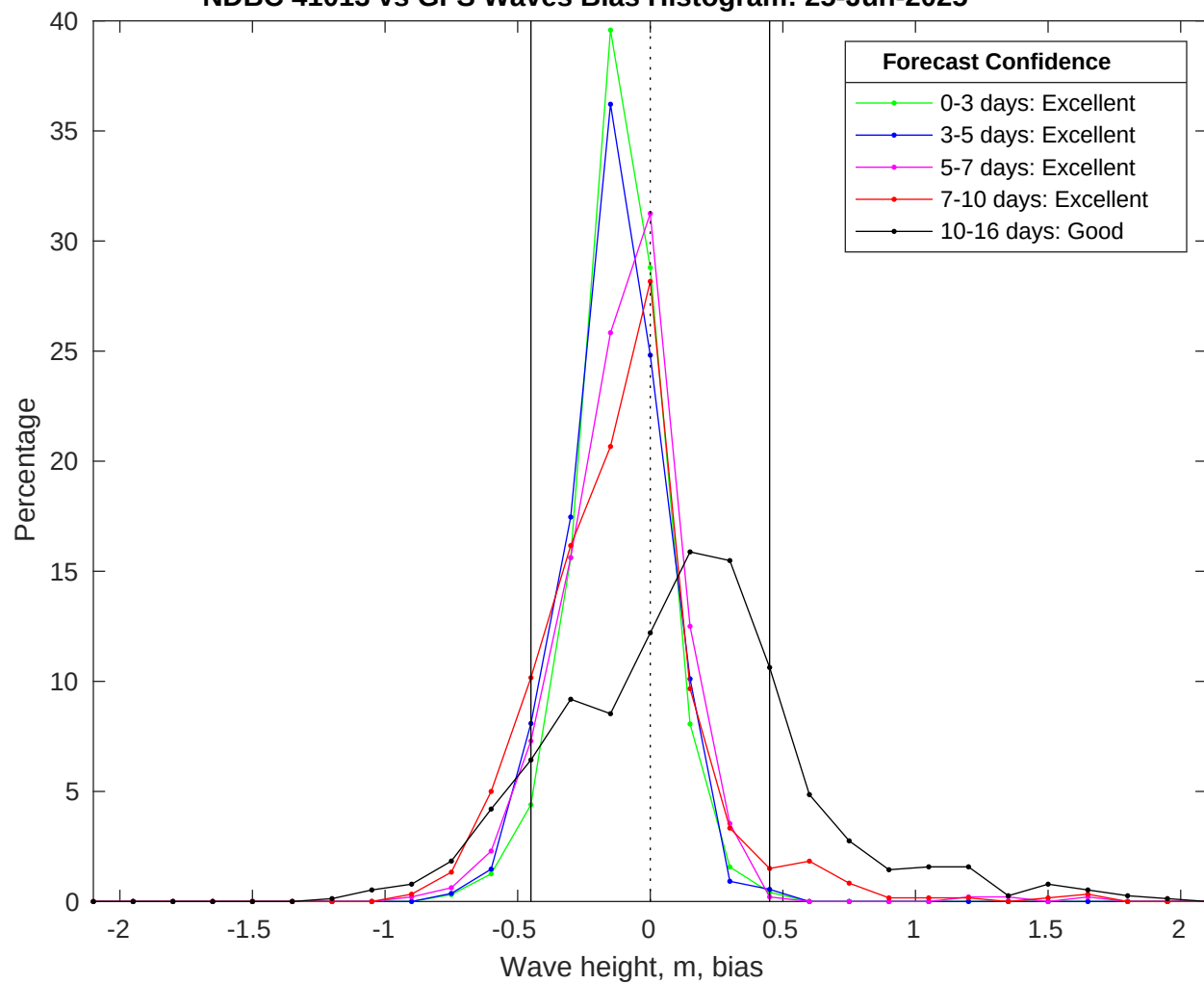
NDBC 41013 vs GFS Waves Bias Histogram: 25-Jun-2025
