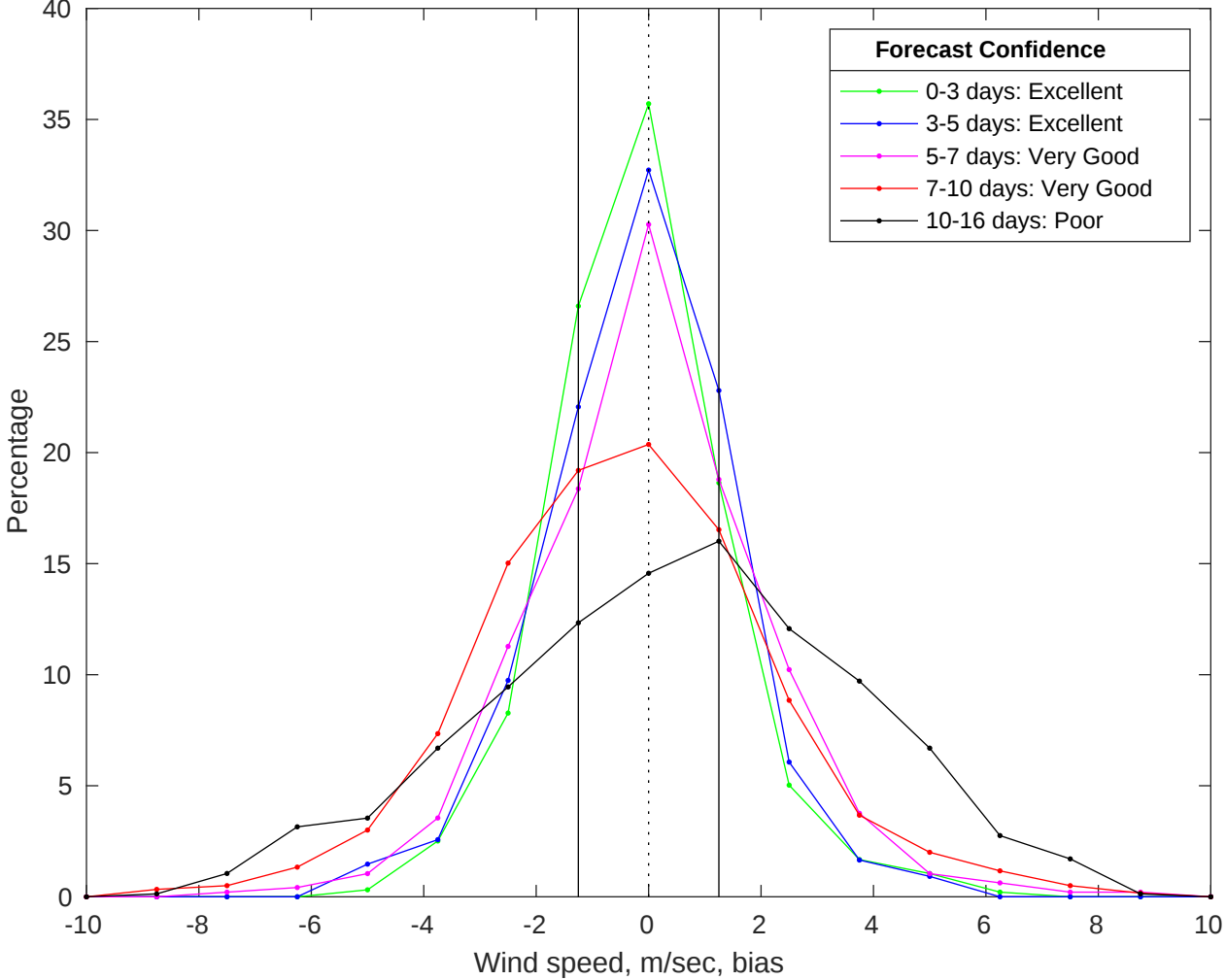
NDBC 41013 vs GFS Winds Bias Histogram: 25-Jun-2025
