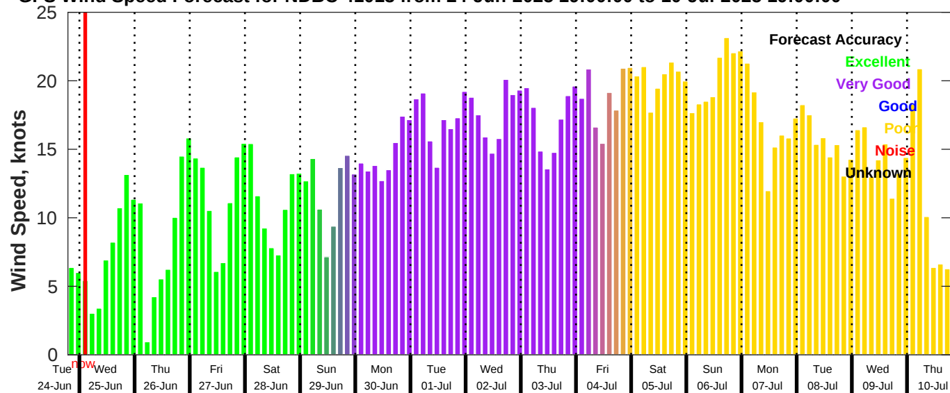
GFS Wind Speed Forecast for NDBC 41013 from 24-Jun-2025 19:00:00 to 10-Jul-2025 19:00:00
