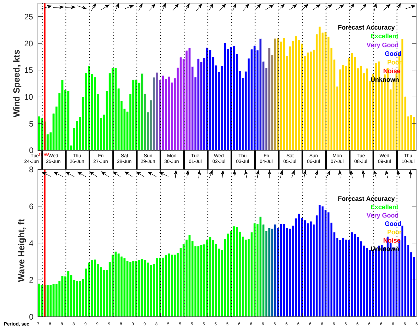
Wind & Wave Forecast for NDBC 41013 from 24-Jun-2025 19:00:00 to 10-Jul-2025 19:00:00
