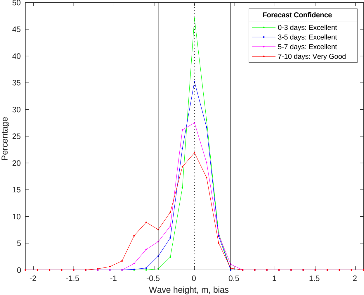
NDBC 41040 vs CMEMS Waves Bias Histogram: 25-Jun-2025
