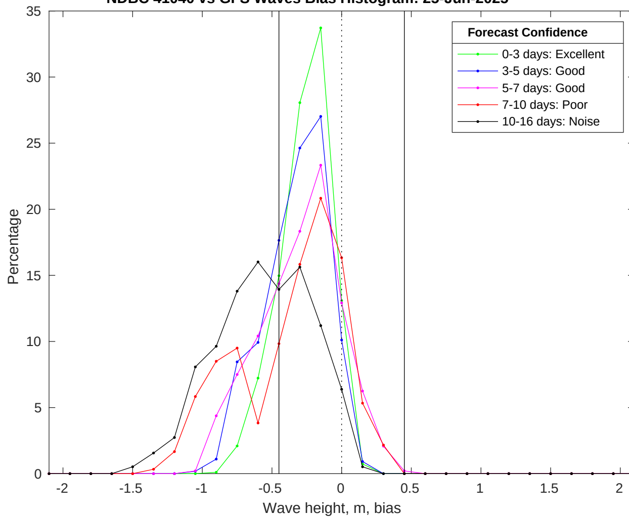
NDBC 41040 vs GFS Waves Bias Histogram: 25-Jun-2025
