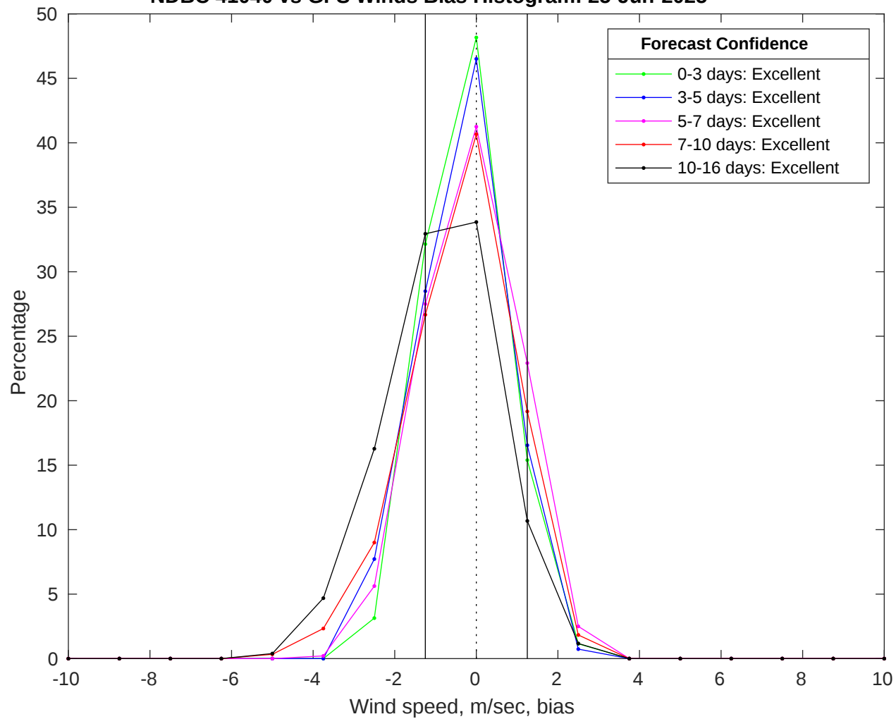
NDBC 41040 vs GFS Winds Bias Histogram: 25-Jun-2025
