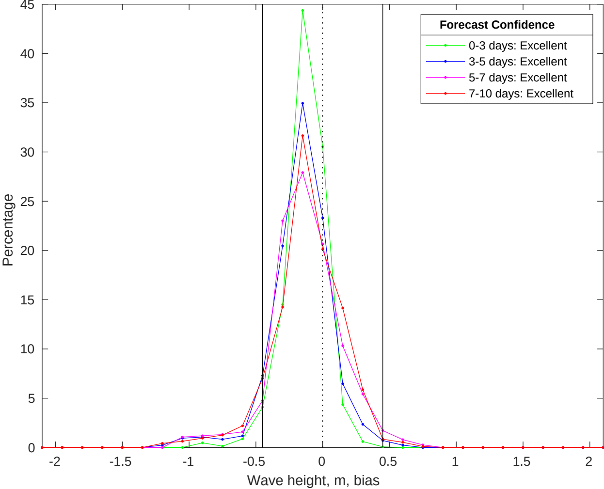
NDBC 42019 vs CMEMS Waves Bias Histogram: 25-Jun-2025
