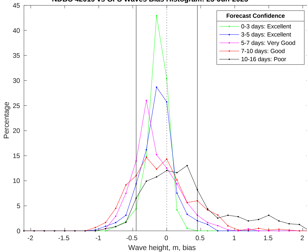
NDBC 42019 vs GFS Waves Bias Histogram: 25-Jun-2025
