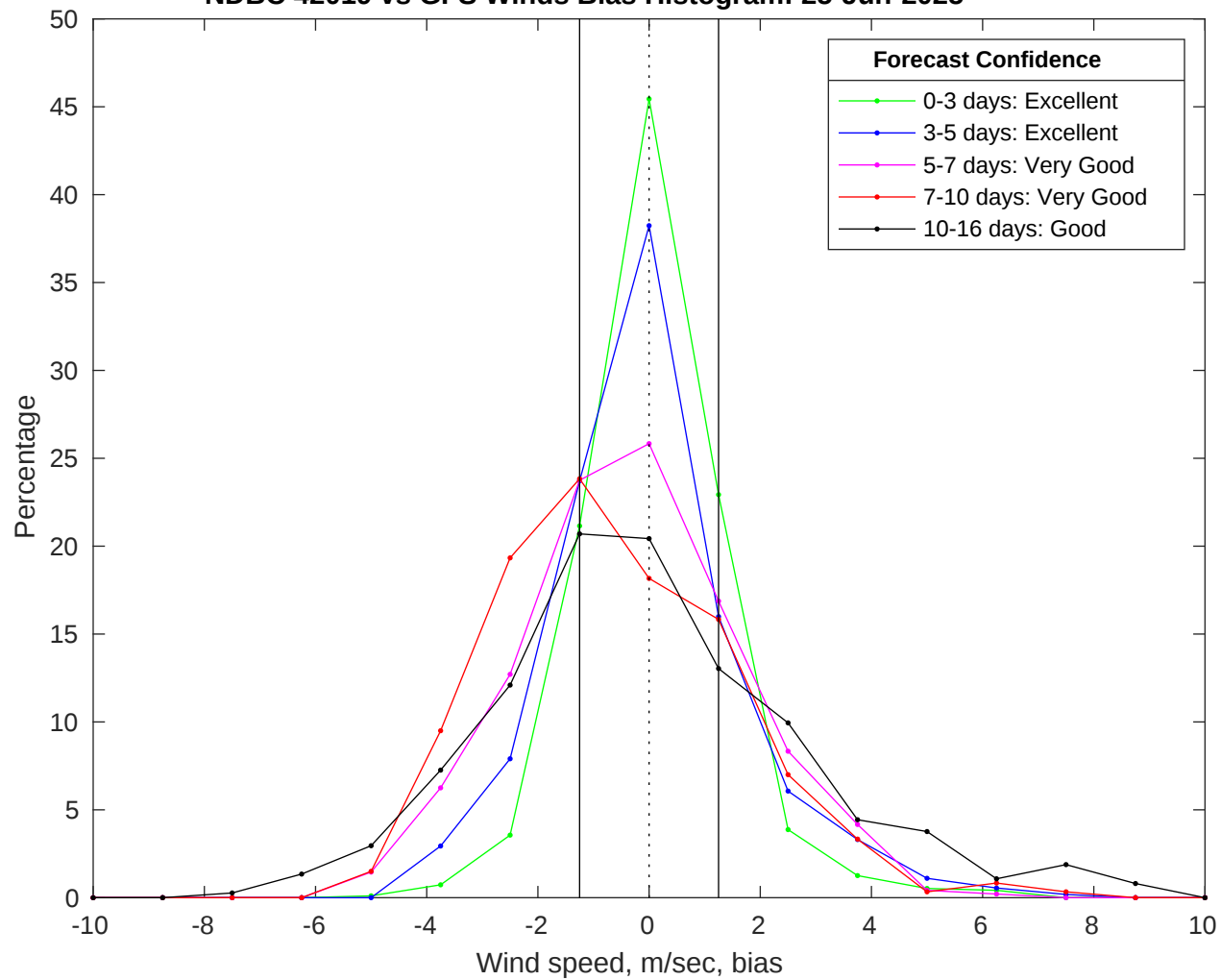
NDBC 42019 vs GFS Winds Bias Histogram: 25-Jun-2025
