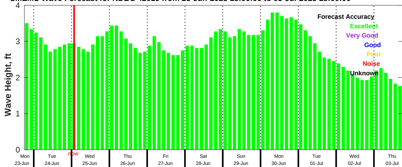
CMEMS Wave Forecast for NDBC 42019 from 23-Jun-2025 18:00:00 to 03-Jul-2025 18:00:00
