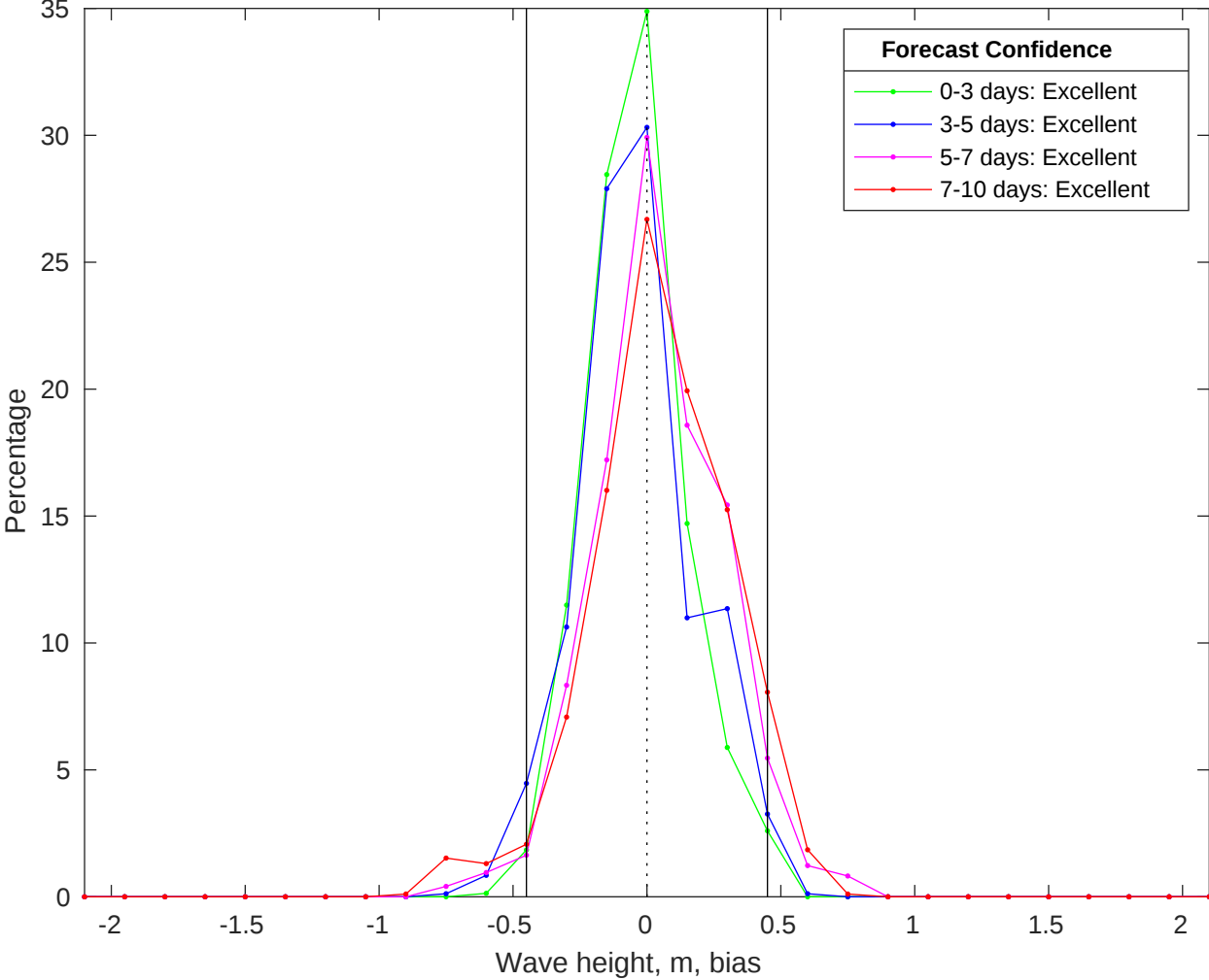
NDBC 42020 vs CMEMS Waves Bias Histogram: 24-Jun-2025
