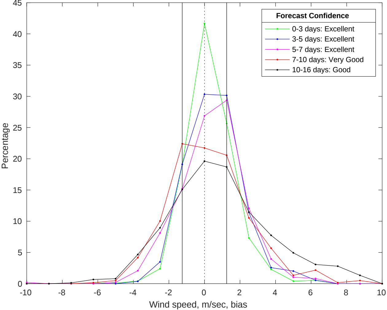
NDBC 42020 vs GFS Winds Bias Histogram: 25-Jun-2025
