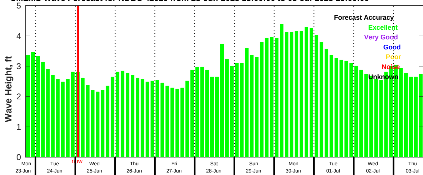
CMEMS Wave Forecast for NDBC 42020 from 23-Jun-2025 18:00:00 to 03-Jul-2025 18:00:00
