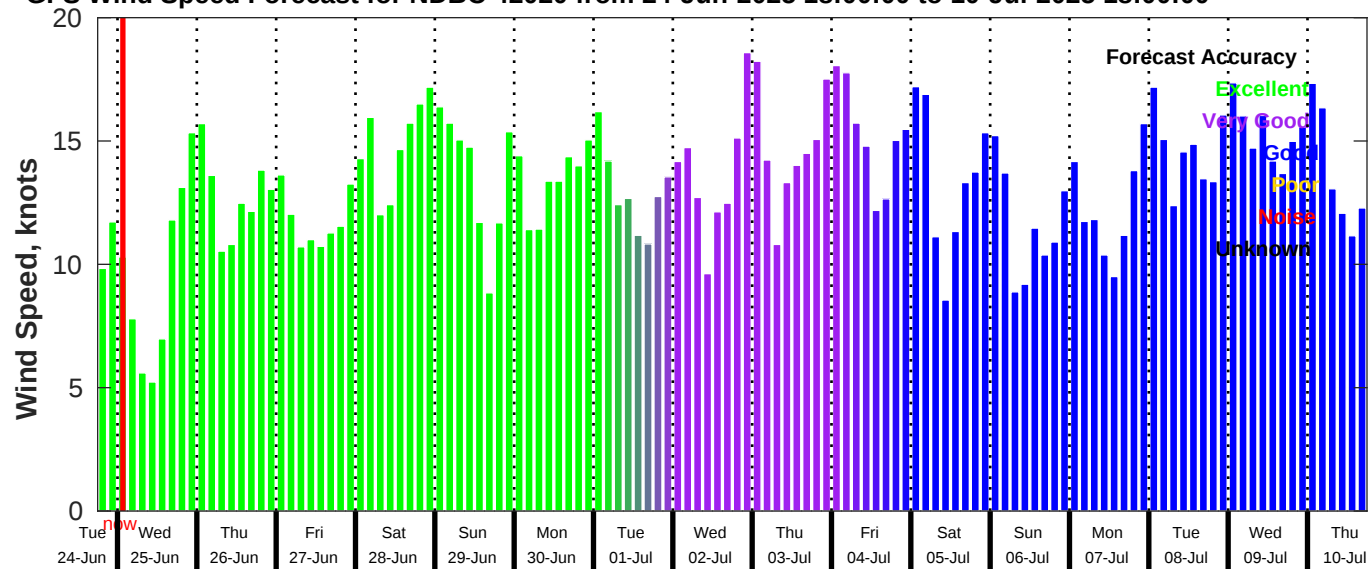
GFS Wind Speed Forecast for NDBC 42020 from 24-Jun-2025 18:00:00 to 10-Jul-2025 18:00:00
