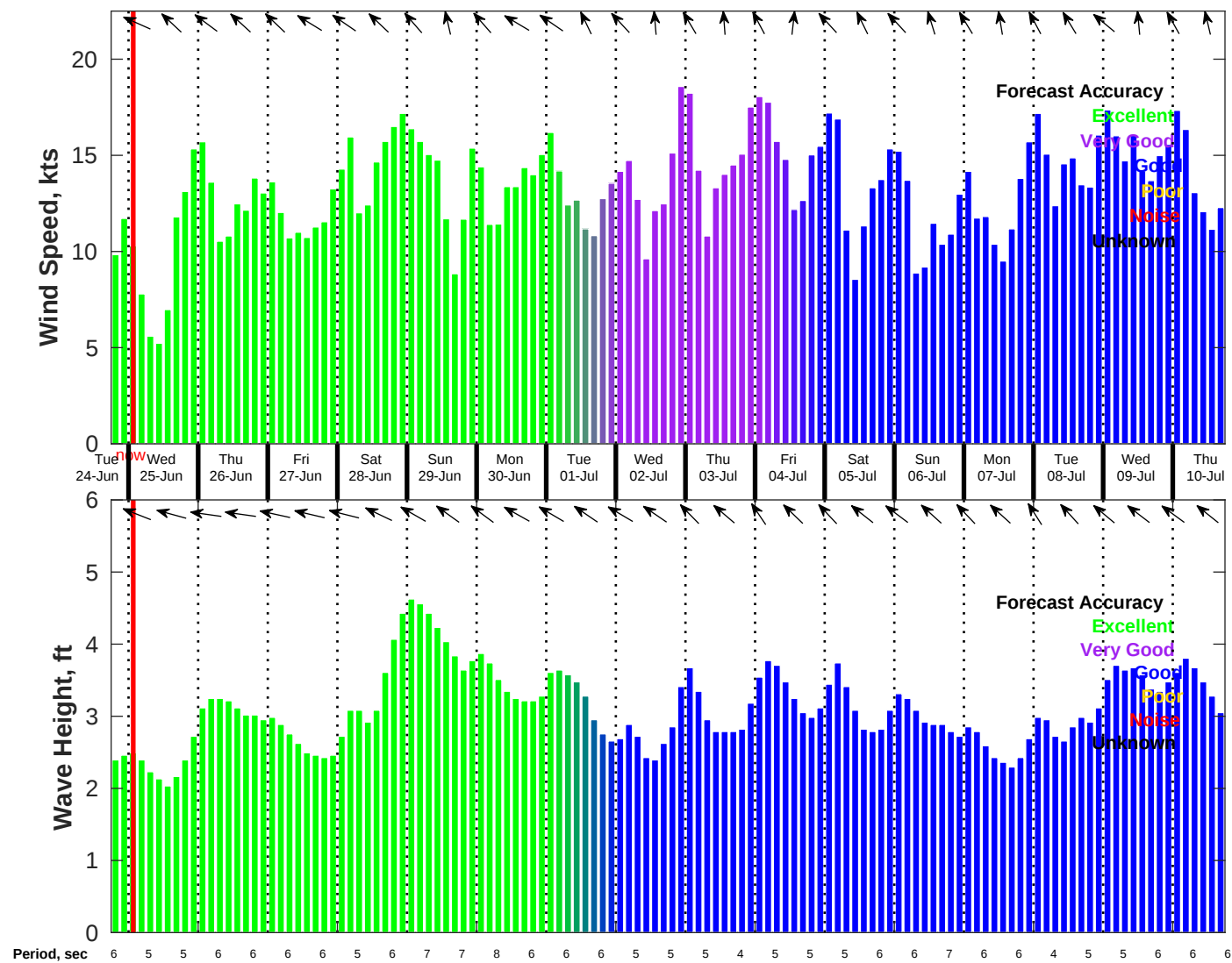
Wind & Wave Forecast for NDBC 42020 from 24-Jun-2025 18:00:00 to 10-Jul-2025 18:00:00
