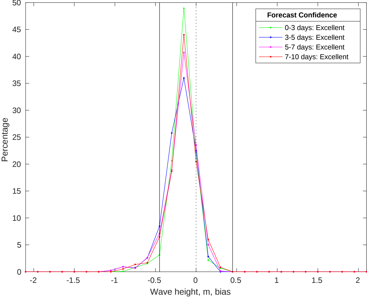
NDBC 42035 vs CMEMS Waves Bias Histogram: 25-Jun-2025
