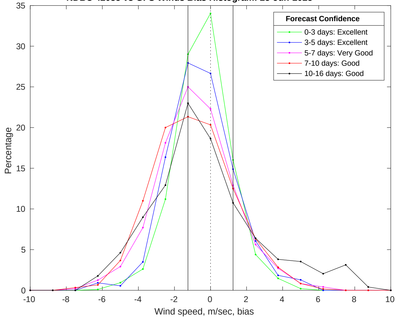
NDBC 42035 vs GFS Winds Bias Histogram: 25-Jun-2025
