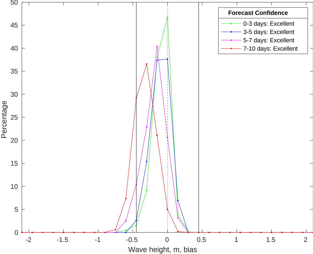
NDBC 42036 vs CMEMS Waves Bias Histogram: 25-Jun-2025
