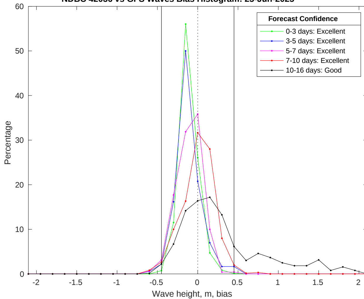
NDBC 42036 vs GFS Waves Bias Histogram: 25-Jun-2025
