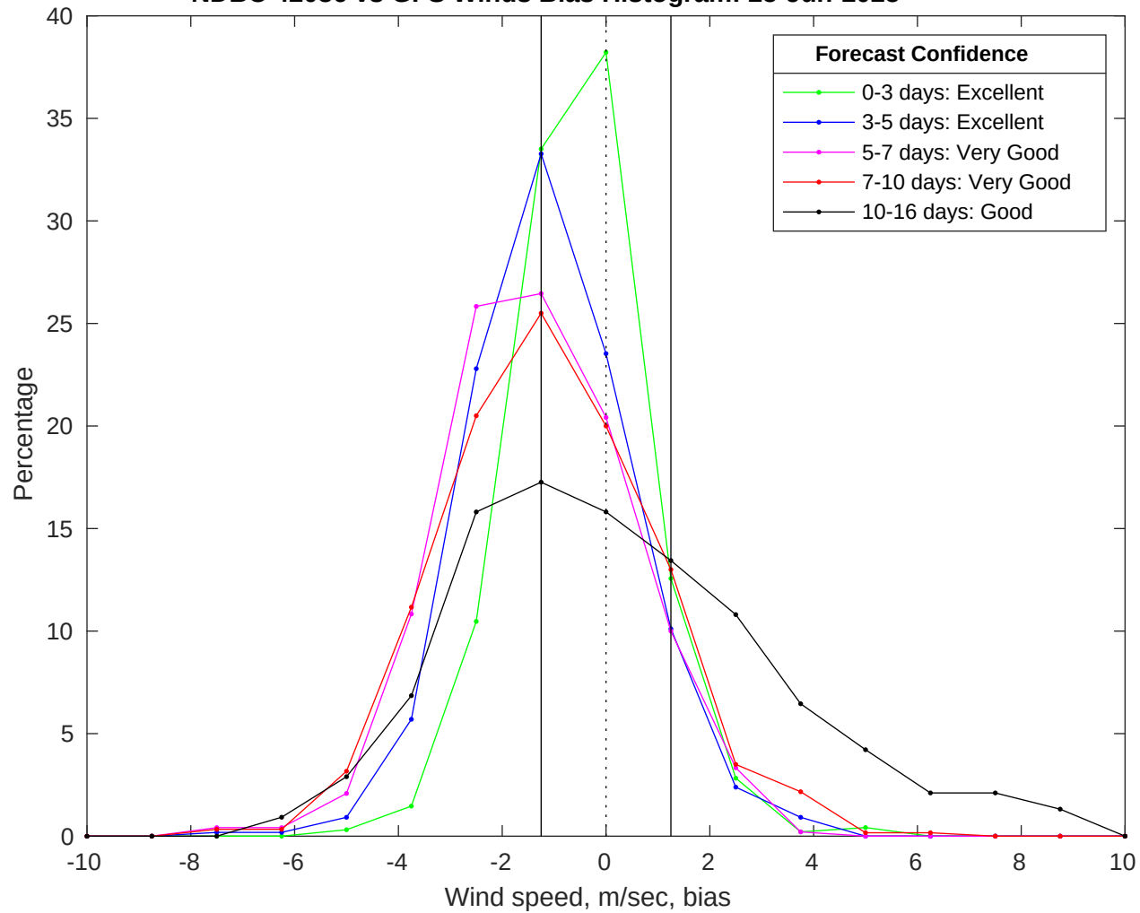
NDBC 42036 vs GFS Winds Bias Histogram: 25-Jun-2025
