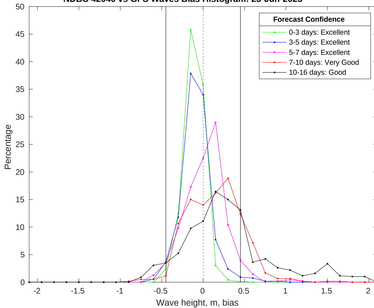
NDBC 42040 vs GFS Waves Bias Histogram: 25-Jun-2025
