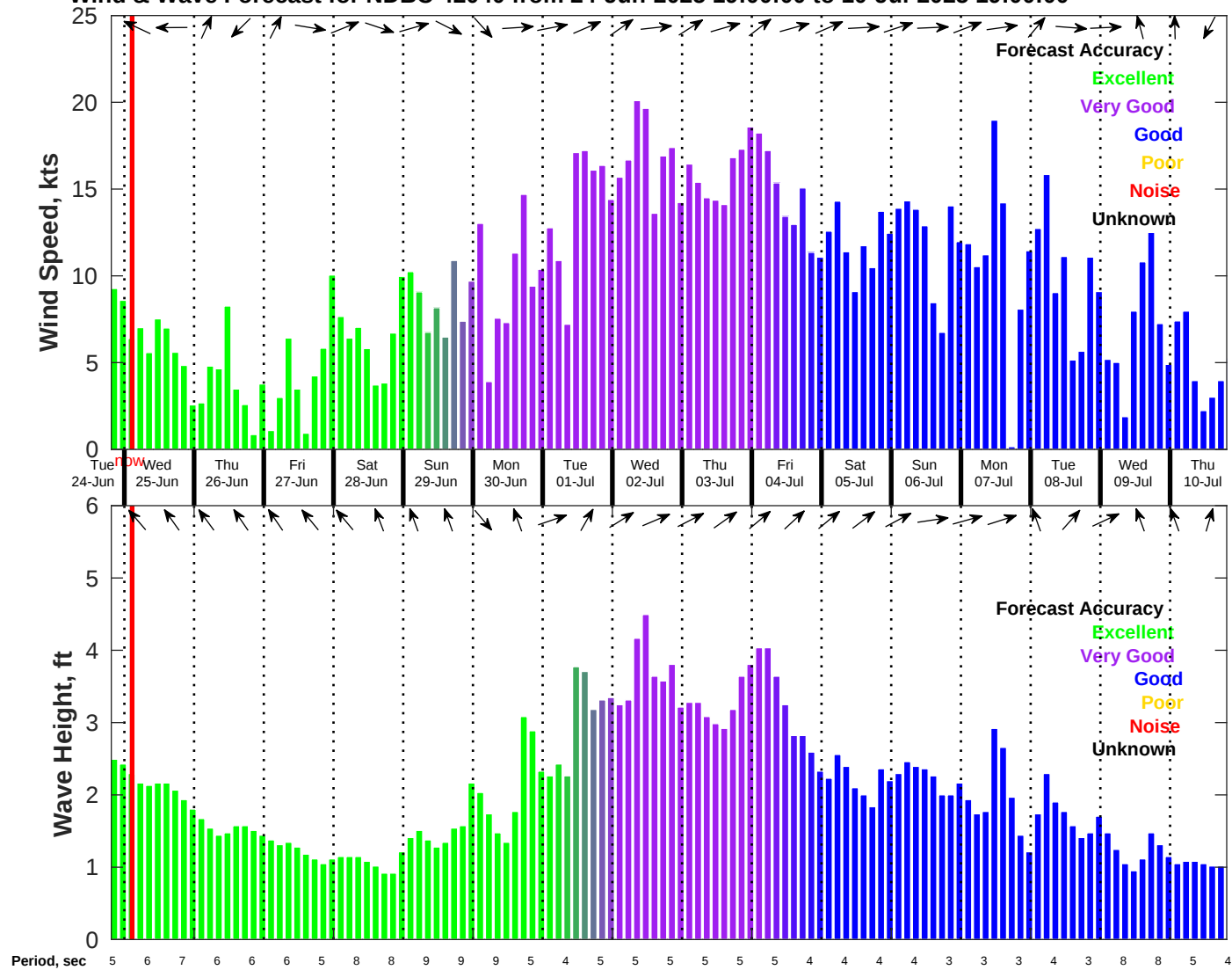
Wind & Wave Forecast for NDBC 42040 from 24-Jun-2025 19:00:00 to 10-Jul-2025 19:00:00
