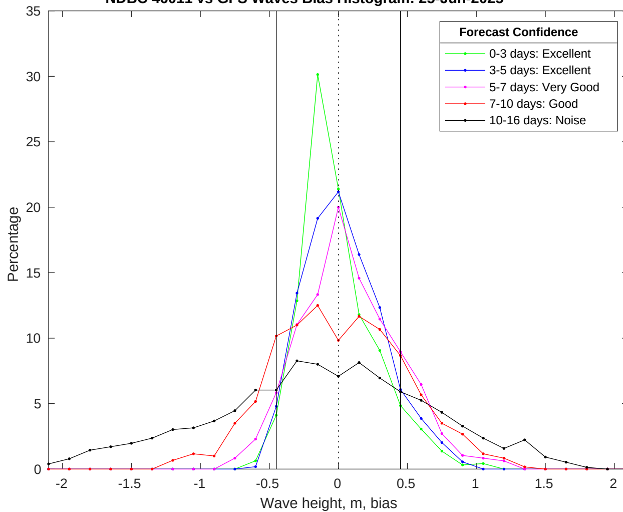
NDBC 46011 vs GFS Waves Bias Histogram: 25-Jun-2025
