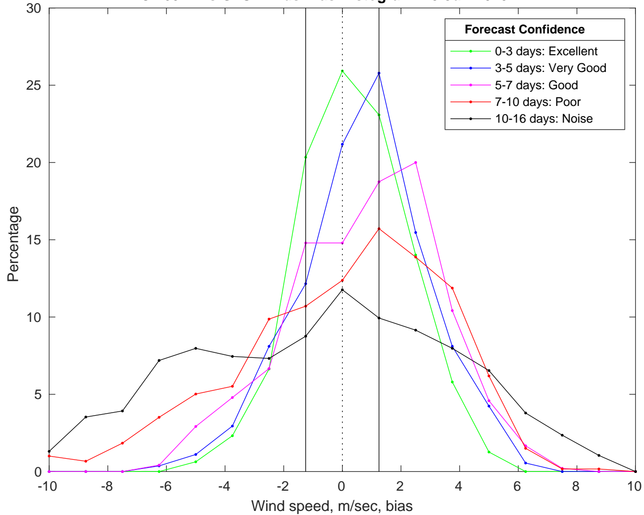
NDBC 46011 vs GFS Winds Bias Histogram: 25-Jun-2025
