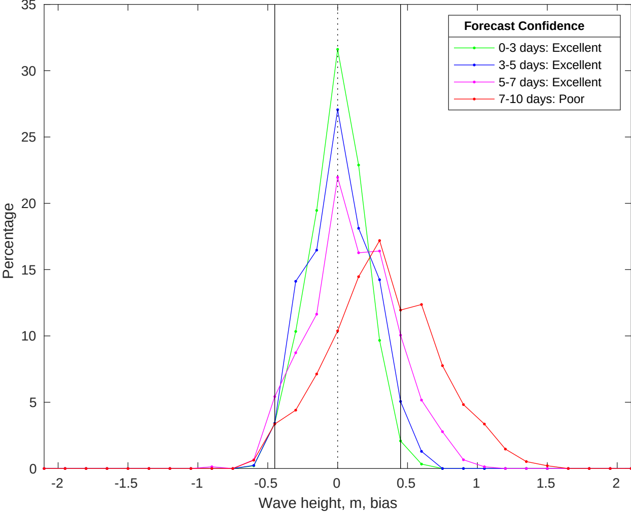
NDBC 46028 vs CMEMS Waves Bias Histogram: 25-Jun-2025
