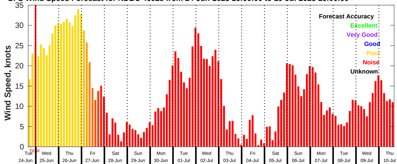
GFS Wind Speed Forecast for NDBC 46028 from 24-Jun-2025 16:00:00 to 10-Jul-2025 16:00:00
