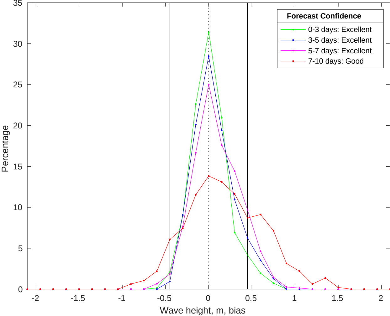
NDBC 46054 vs CMEMS Waves Bias Histogram: 25-Jun-2025
