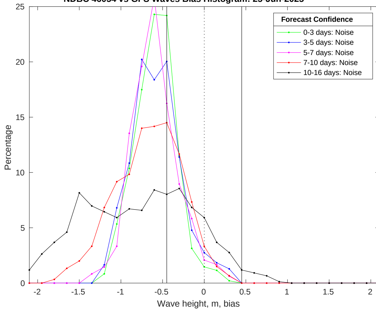
NDBC 46054 vs GFS Waves Bias Histogram: 25-Jun-2025
