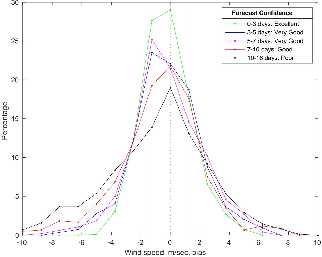
NDBC 46054 vs GFS Winds Bias Histogram: 25-Jun-2025
