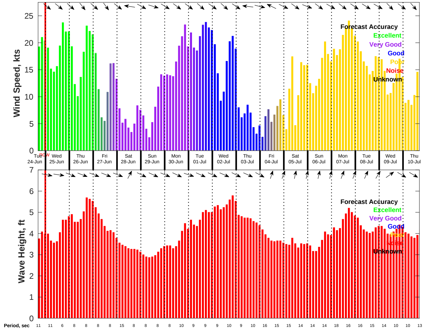
Wind & Wave Forecast for NDBC 46054 from 24-Jun-2025 16:00:00 to 10-Jul-2025 16:00:00
