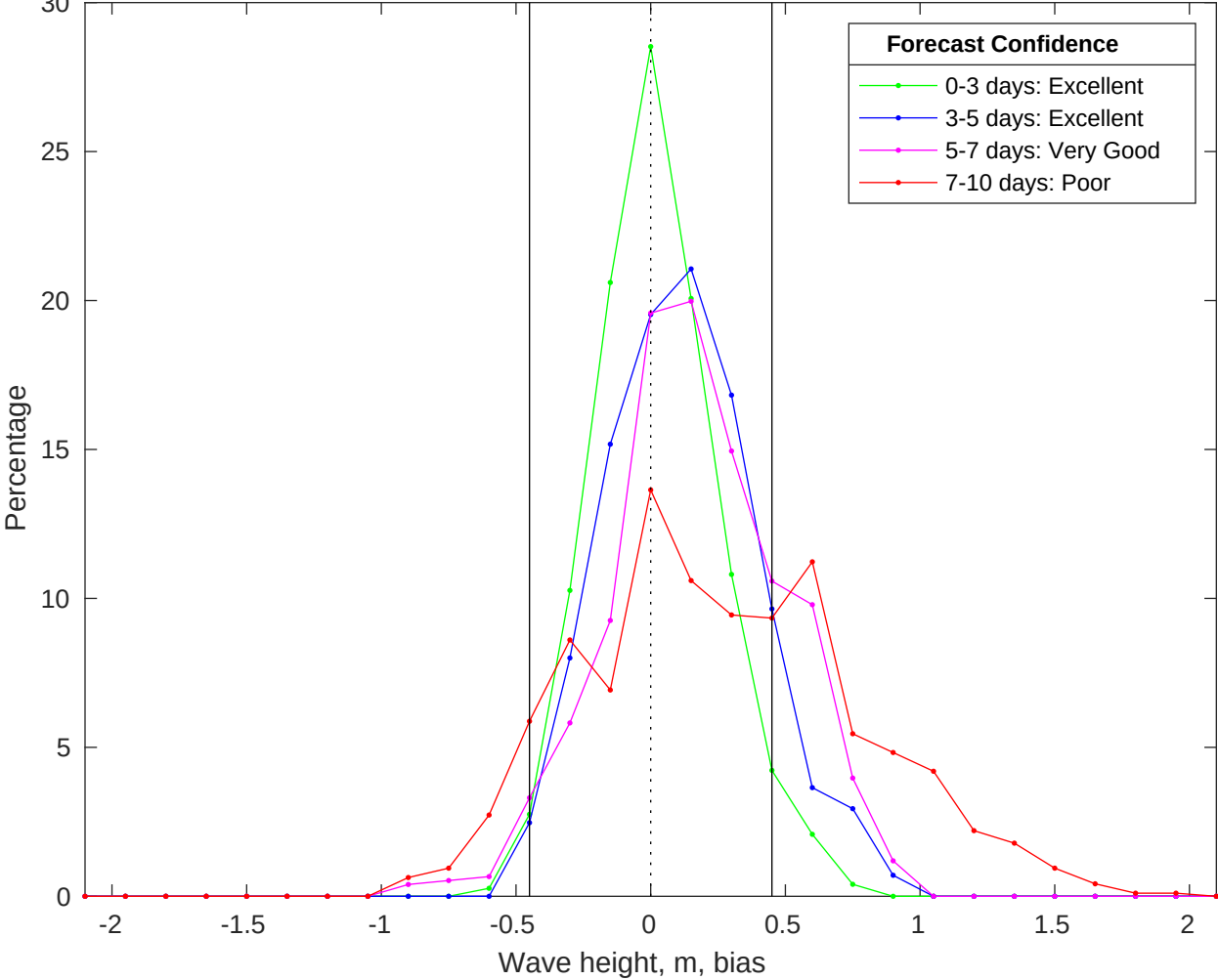
NDBC 46069 vs CMEMS Waves Bias Histogram: 25-Jun-2025
