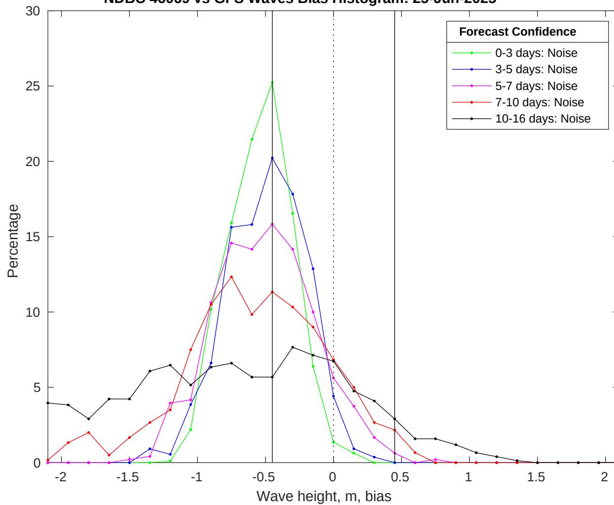
NDBC 46069 vs GFS Waves Bias Histogram: 25-Jun-2025
