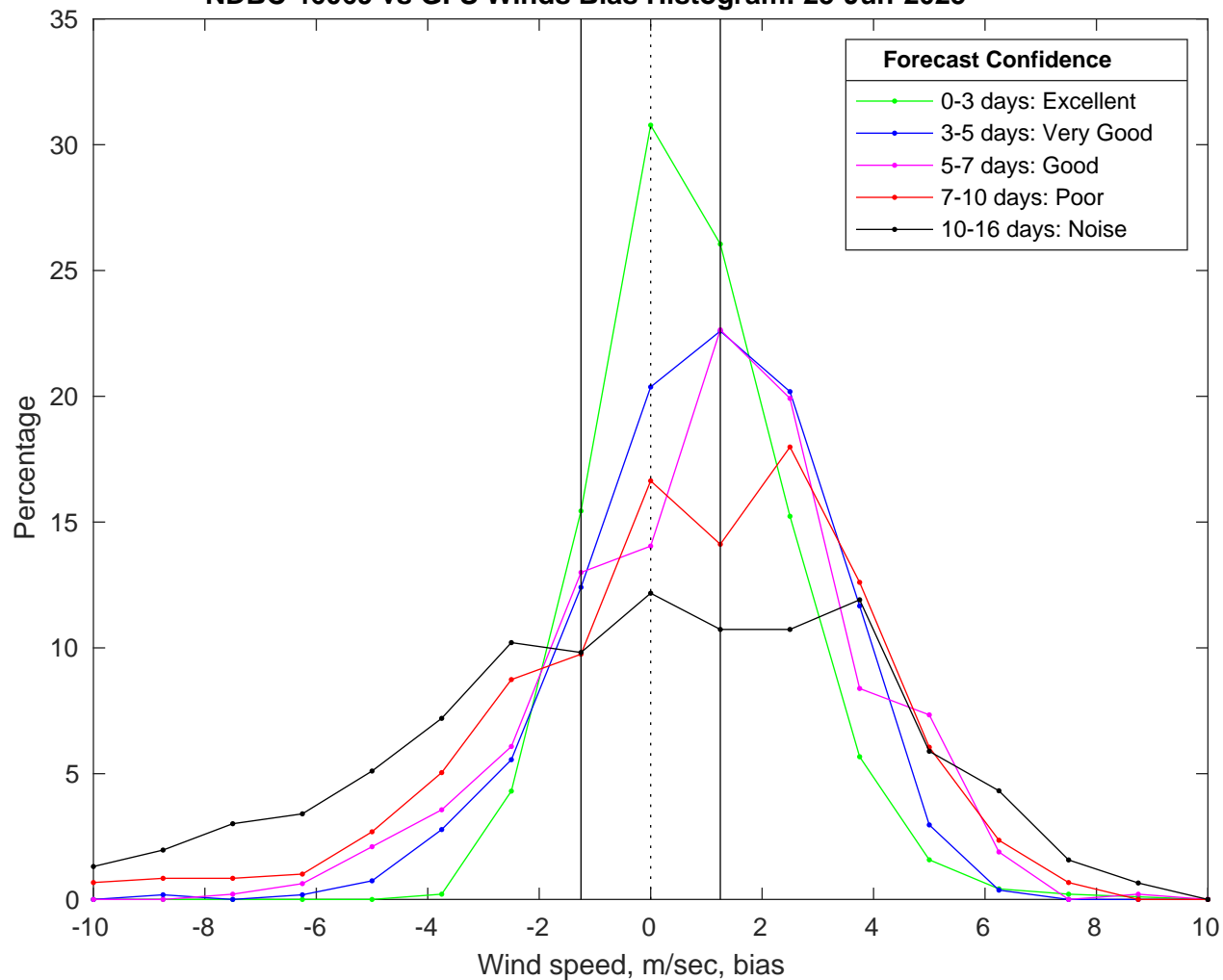
NDBC 46069 vs GFS Winds Bias Histogram: 25-Jun-2025
