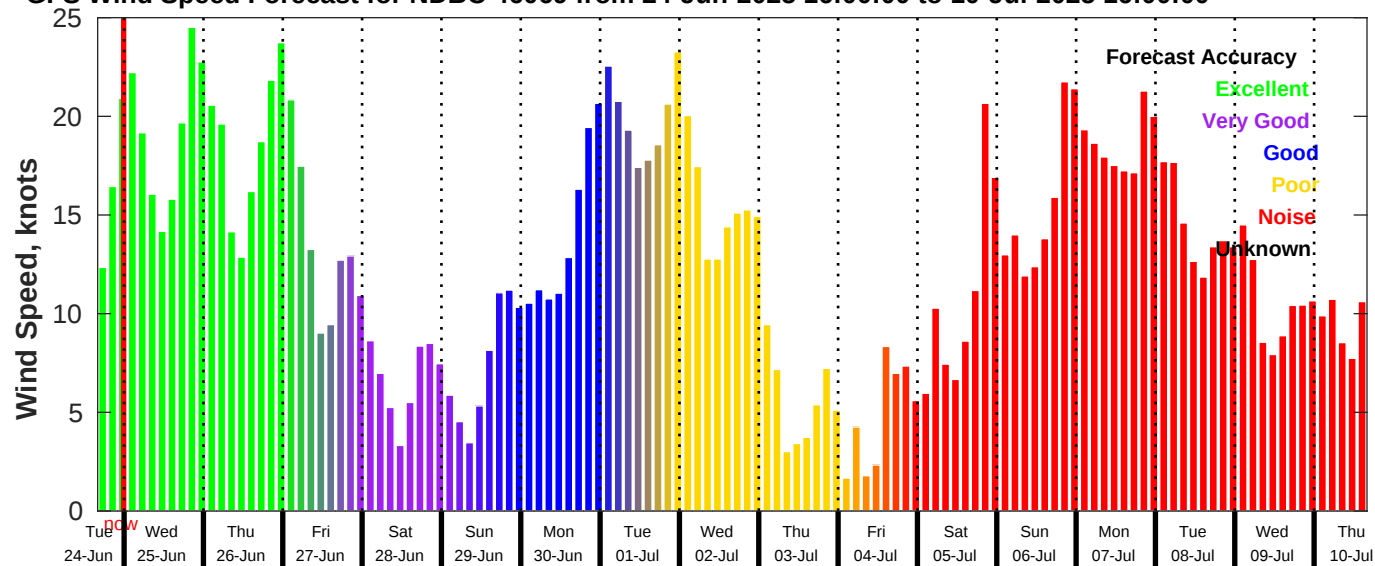
GFS Wind Speed Forecast for NDBC 46069 from 24-Jun-2025 16:00:00 to 10-Jul-2025 16:00:00
