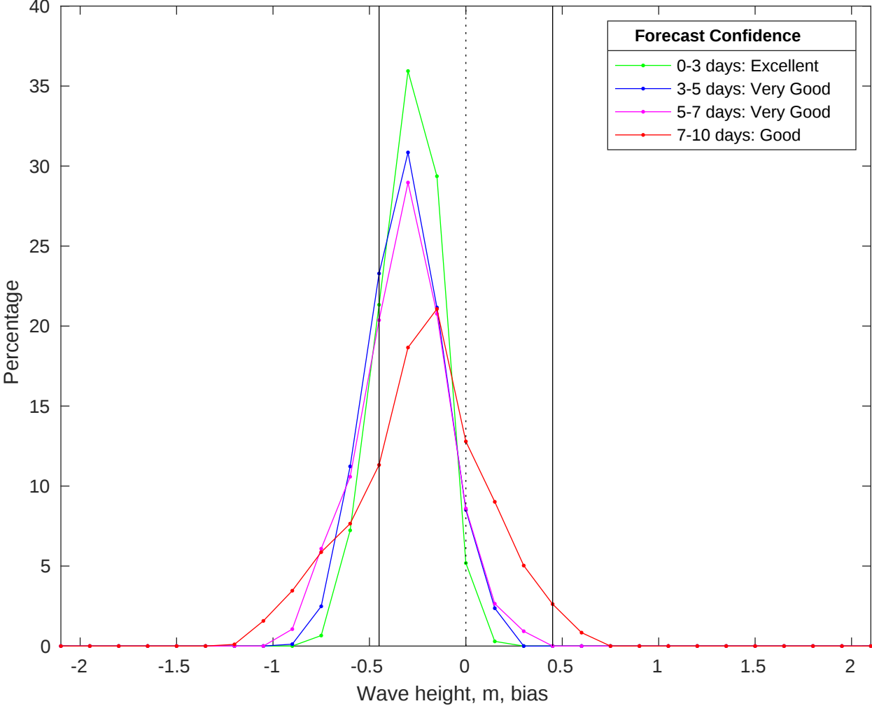
NDBC 51209 vs CMEMS Waves Bias Histogram: 25-Jun-2025
