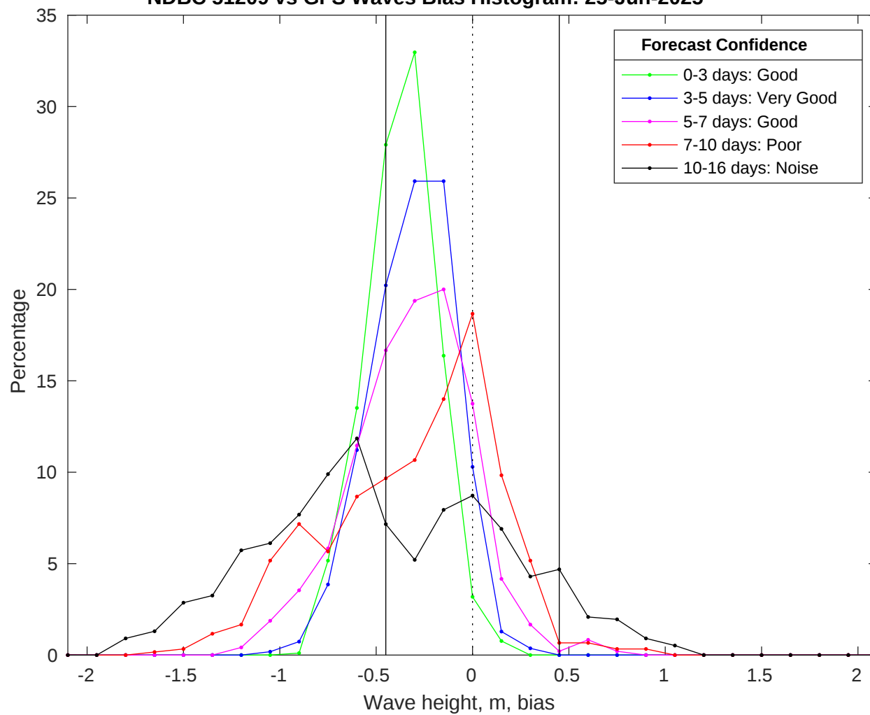
NDBC 51209 vs GFS Waves Bias Histogram: 25-Jun-2025
